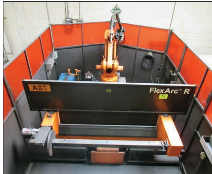
ABB Flexarc R Mdl. IRB1400 M2000 Robotic Welding Cell
