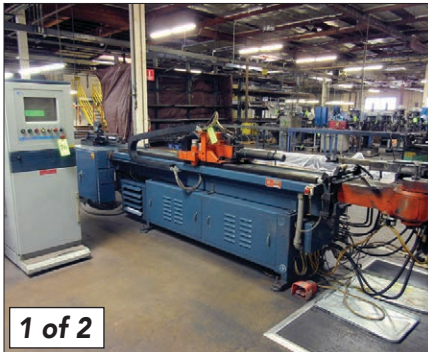
Eaton Leonard Mdl. Vb 200 SE CNC Tube Bender
